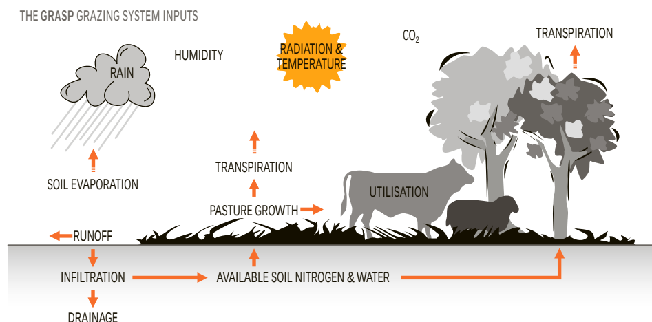
Figure 4.1 Schematic representation of the GRASP pasture model
