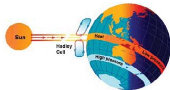
Figure 1.1 Atmospheric wind and pressure systems
